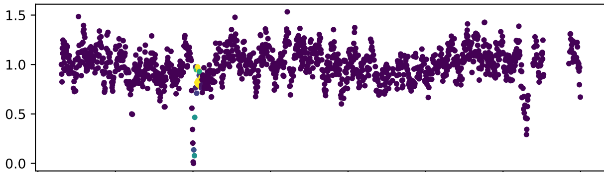
Single Model Predictions - KIC 3542116
